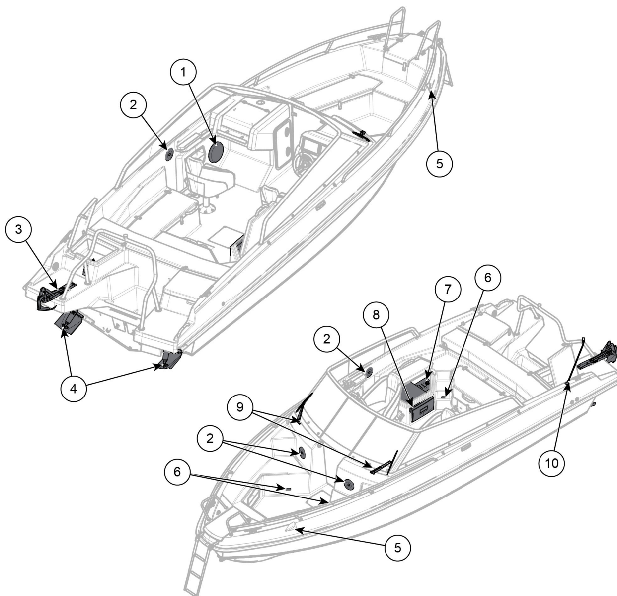
Figure 8.2 Cross 75 BR electrical equipment
