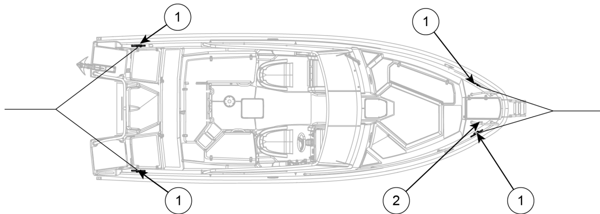
Figure 5.6 Cross 75 BR mooring and towing points
