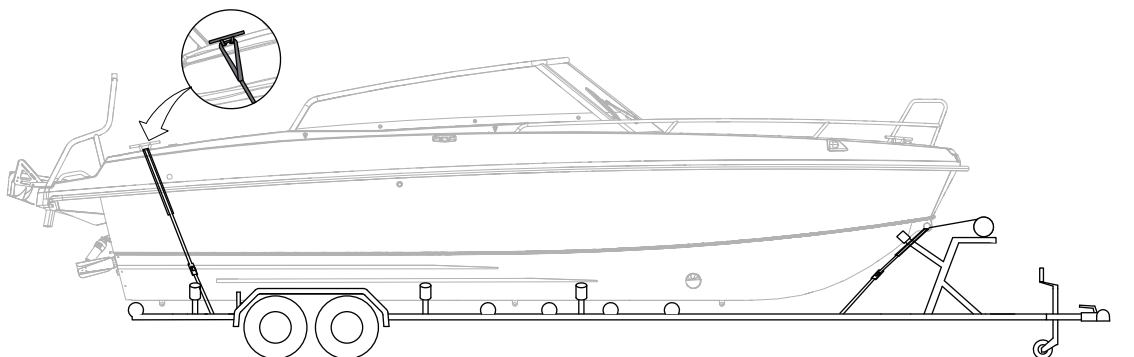
Figure 12.1 Cross 75 BR trailer transportation
