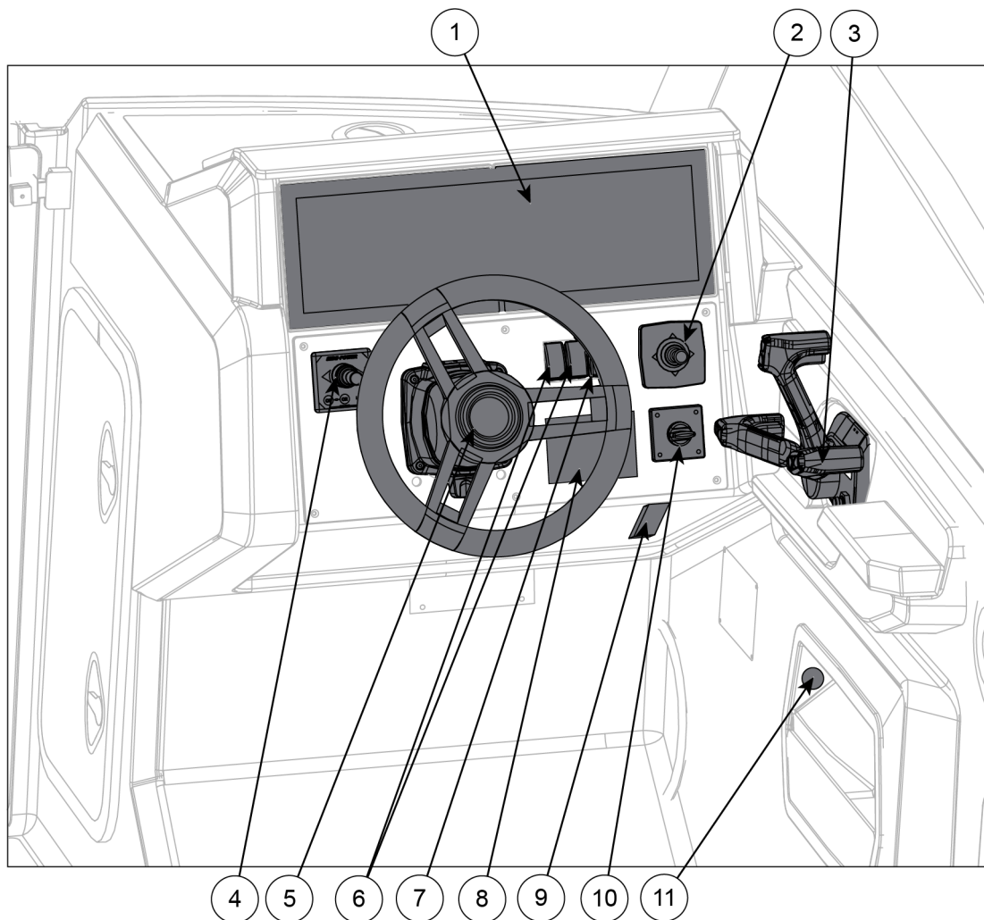
Figure 5.1 Cross 75 BR helm station controls
