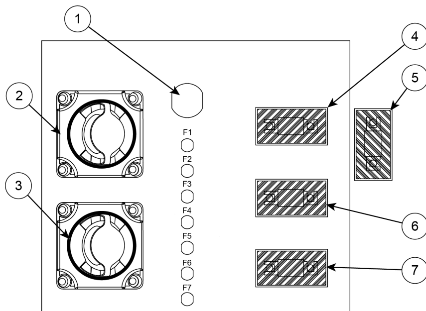
Figure 8.1 Cross 75 BR main switch and fuse panel
