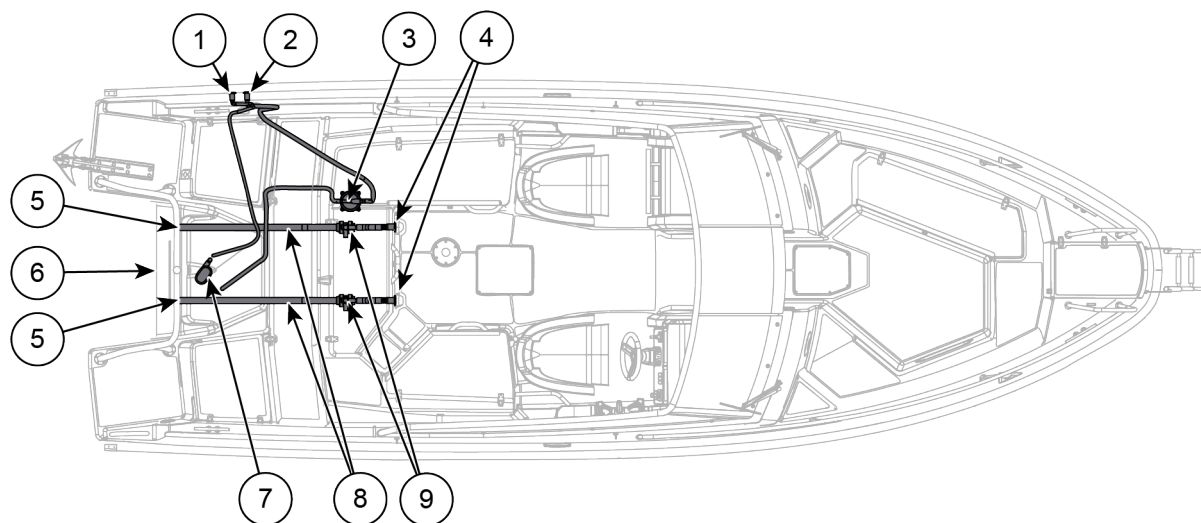
Figure 9.1 Cross 75 BR bilge pumps and draining
