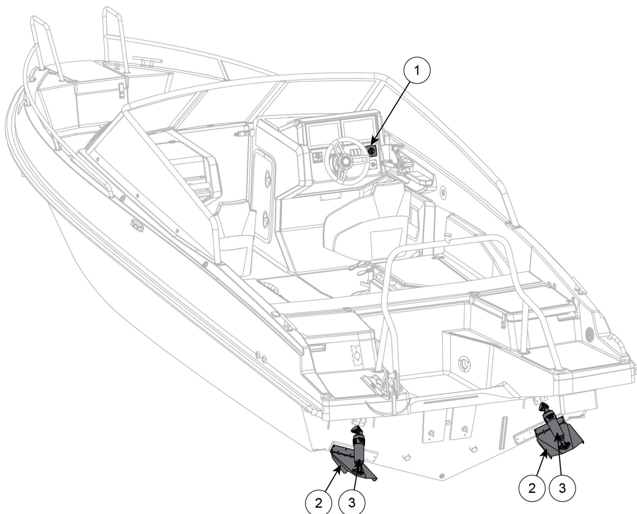
Figure 5.5 Cross 75 BR trim system
