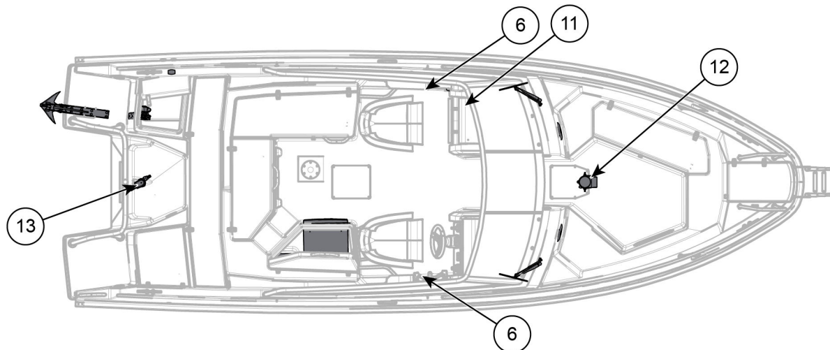
Figure 8.3 Cross 75 BR electrical equipment
