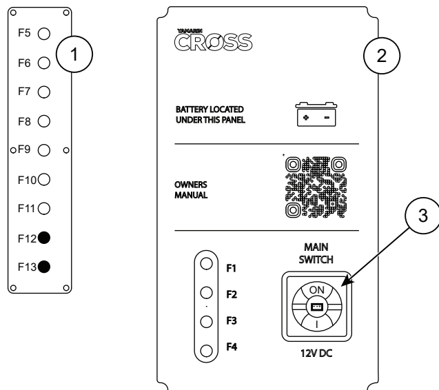
Figure 8.1 Cross 55 BR main switch and fuse panel
