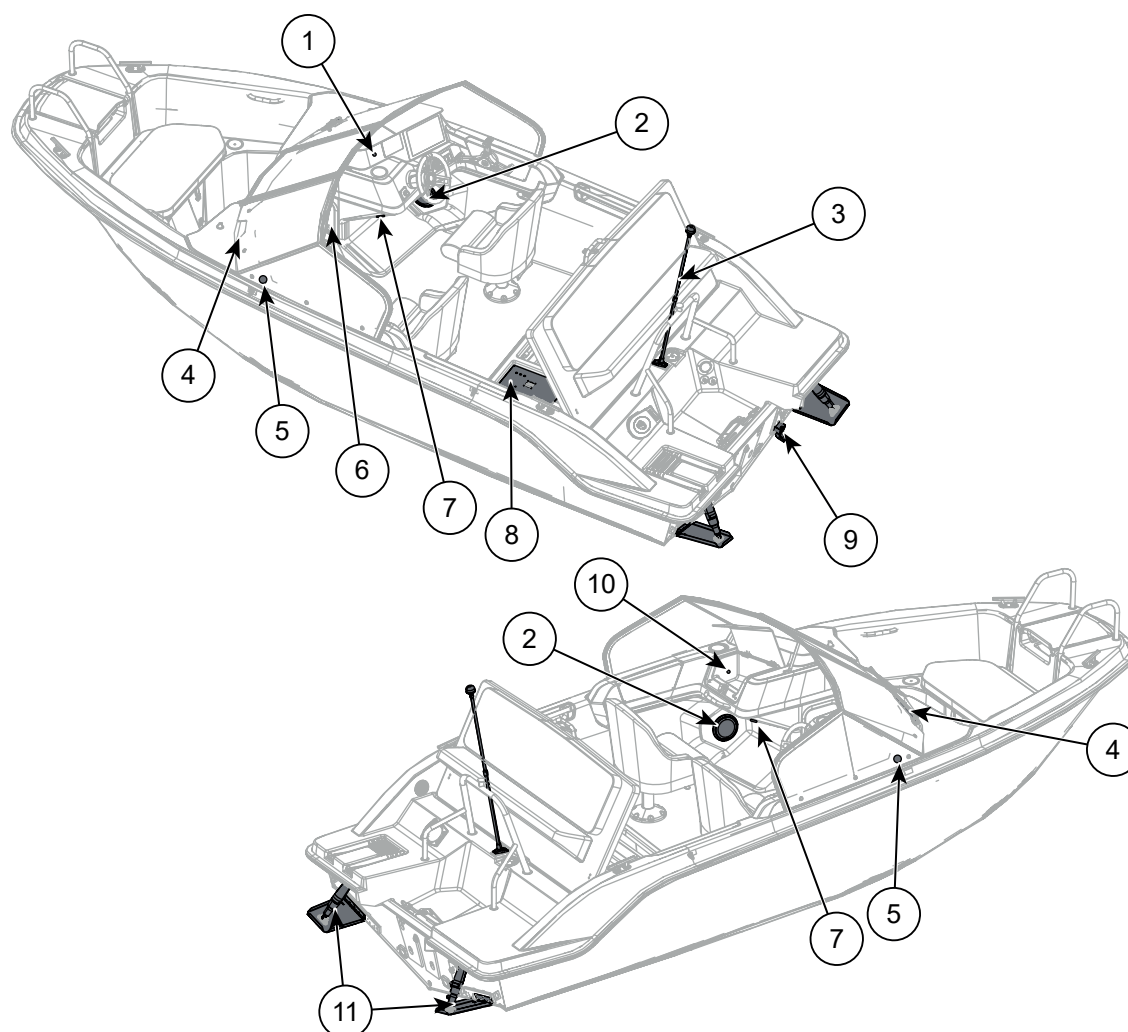
Figure 8.3 Cross 55 BR electrical equipment
