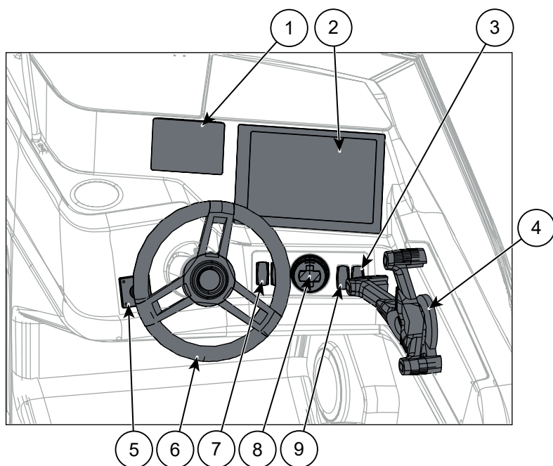
Figure 5.1 Cross 55 BR helm station controls
