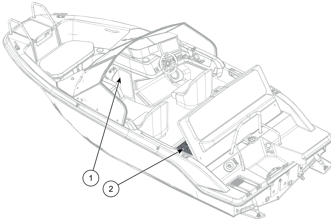
Figure 8.2 Cross 55 BR fuse panel locations
