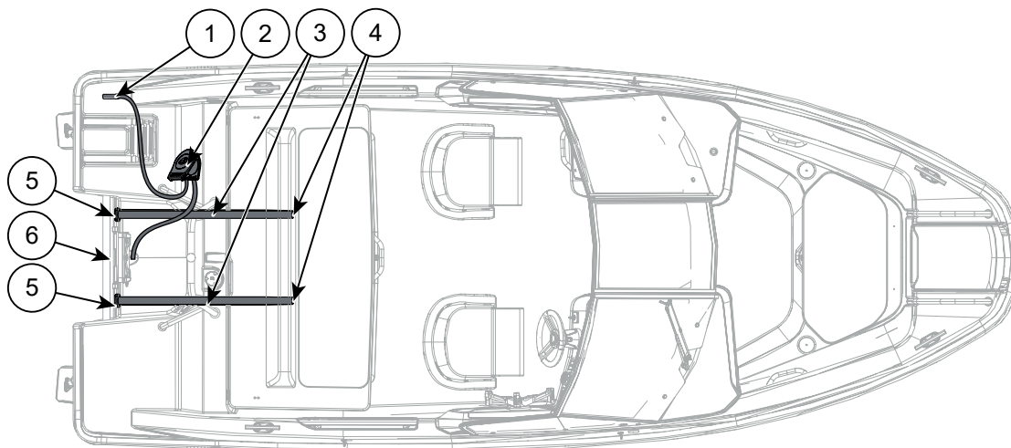
Figure 9.1 Cross 55 BR bilge pumps and draining
