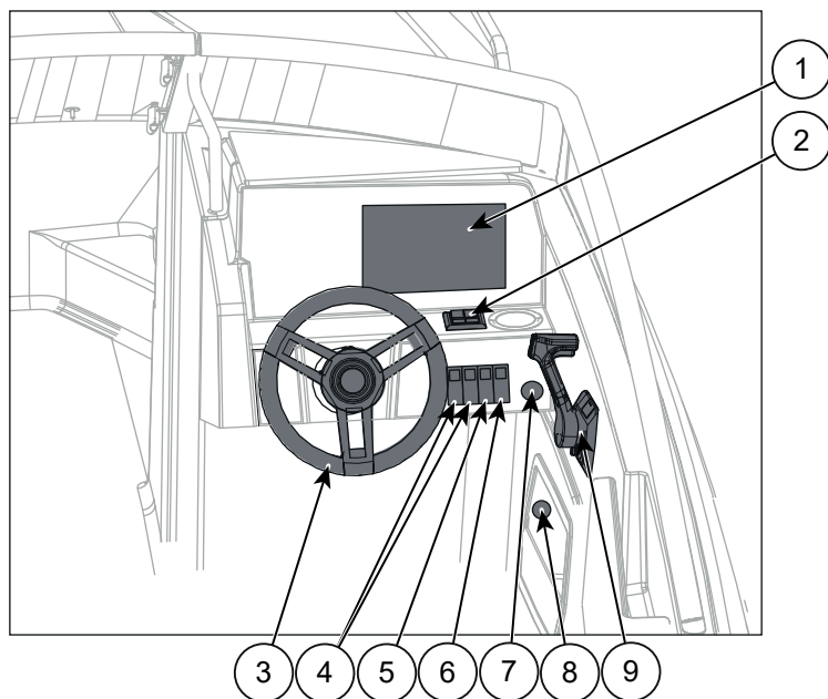
Figure 5.1 Cross 64 BR helm station controls
