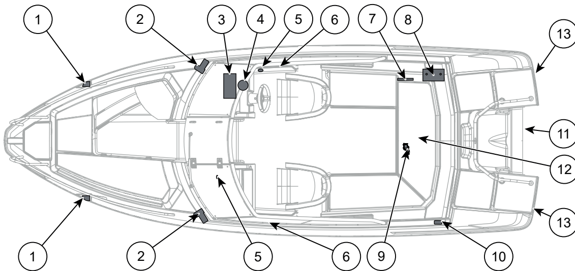
Figure 8.2 Cross 64 BR electrical equipment
