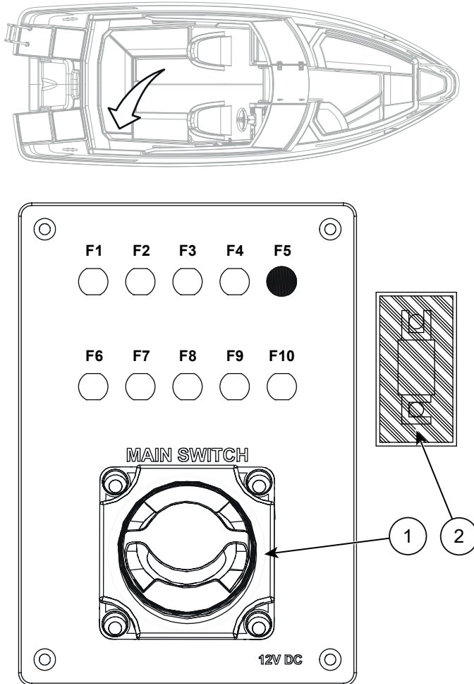
Figure 8.1 Cross 64 BR main switch and fuse panel
