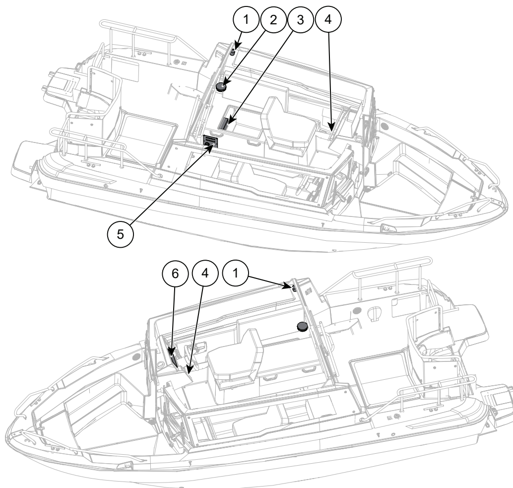
Figure 8.3 Cross 60 Cabin electrical equipment
