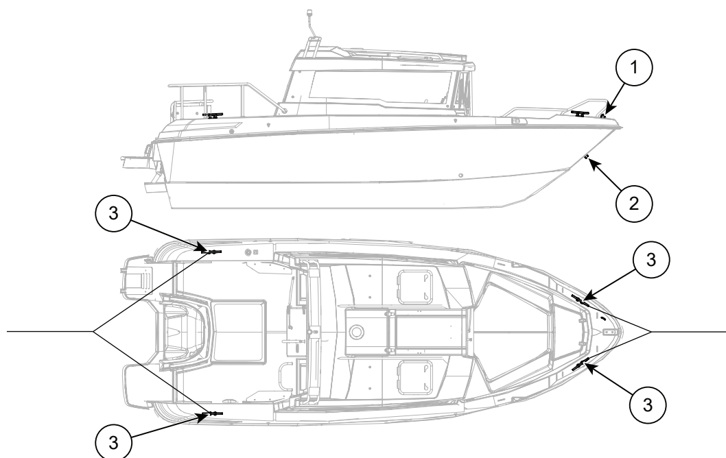
Figure 5.7 Cross 60 Cabin mooring and towing points
