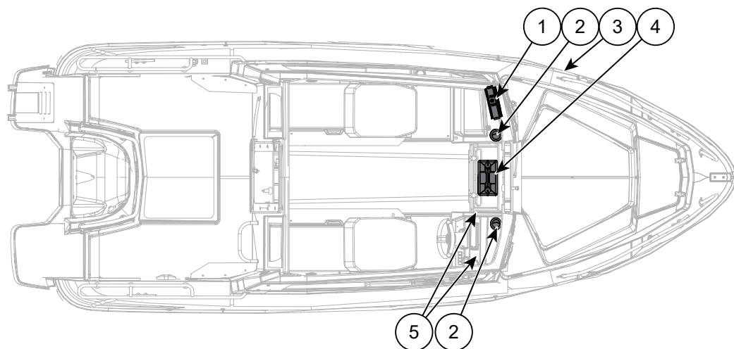
Figure 6.2 Cross 60 Cabin heating system
