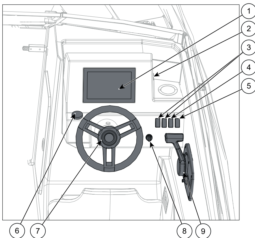
Figure 5.1 Cross 62 BR helm station controls
