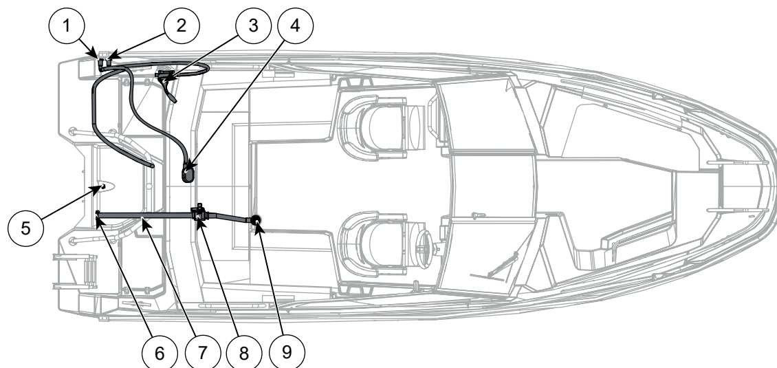
Figure 9.1 Cross 62 BR bilge pumps and draining
