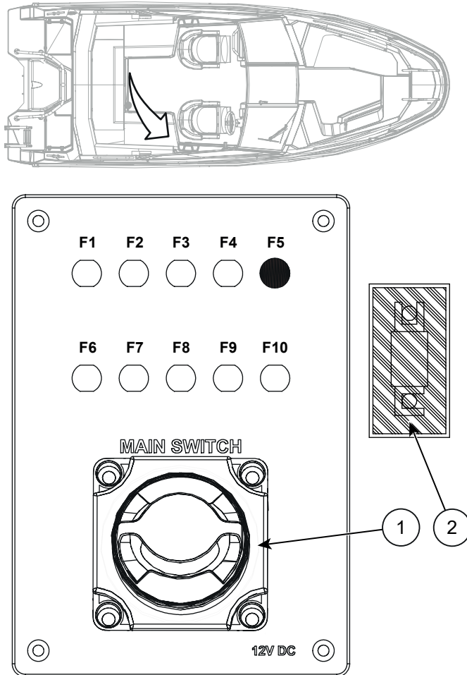
Figure 8.1 Cross 62 BR main switch and fuse panel
