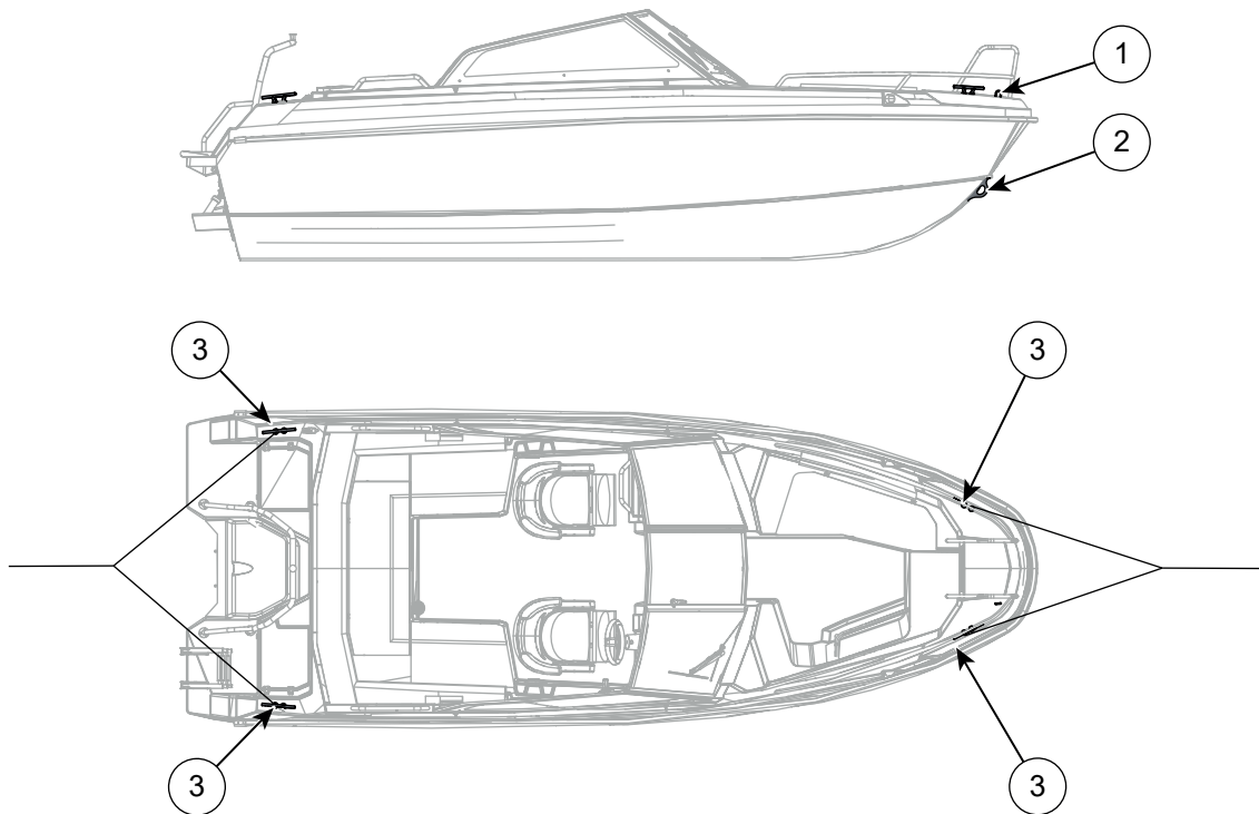
Figure 5.5 Cross 62 BR mooring and towing points
