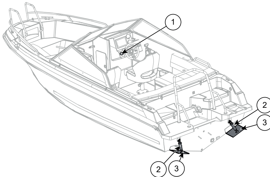
Figure 5.4 Cross 62 BR trim system
